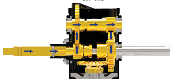
Low Gear
