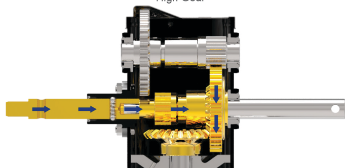
High Gear
